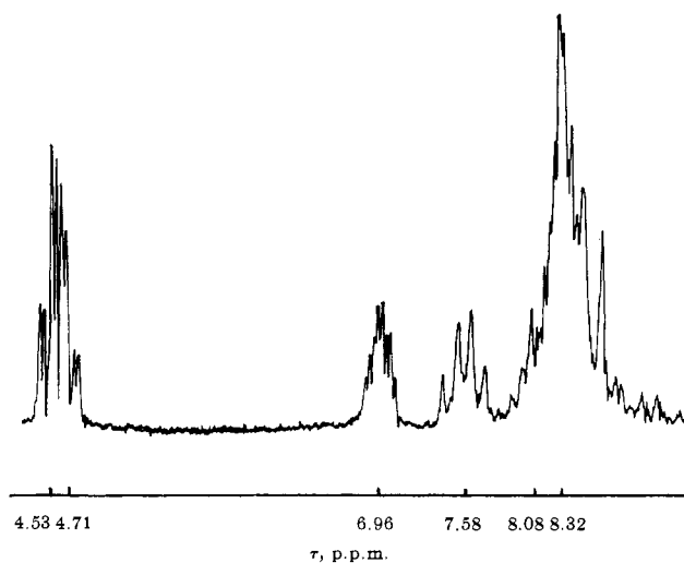
Fig. 1.—Nuclear magnetic resonance (60 Mc.) spectrum of VI in deuterochloroform. Resonance positions are given as \tau -values (p.p.m.) relative to internal tetramethylsilane. The spectrum was run on a degassed sample sealed under vacuum to exclude oxygen.
